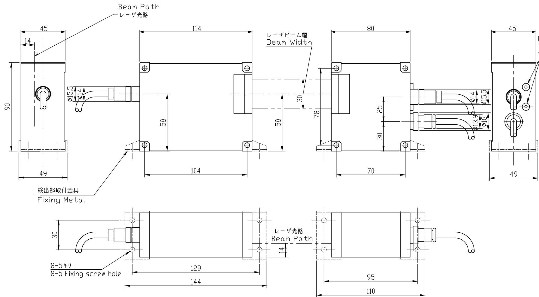
LDM-303H-SP/303HS-SP 外形図 OutLine Dra
