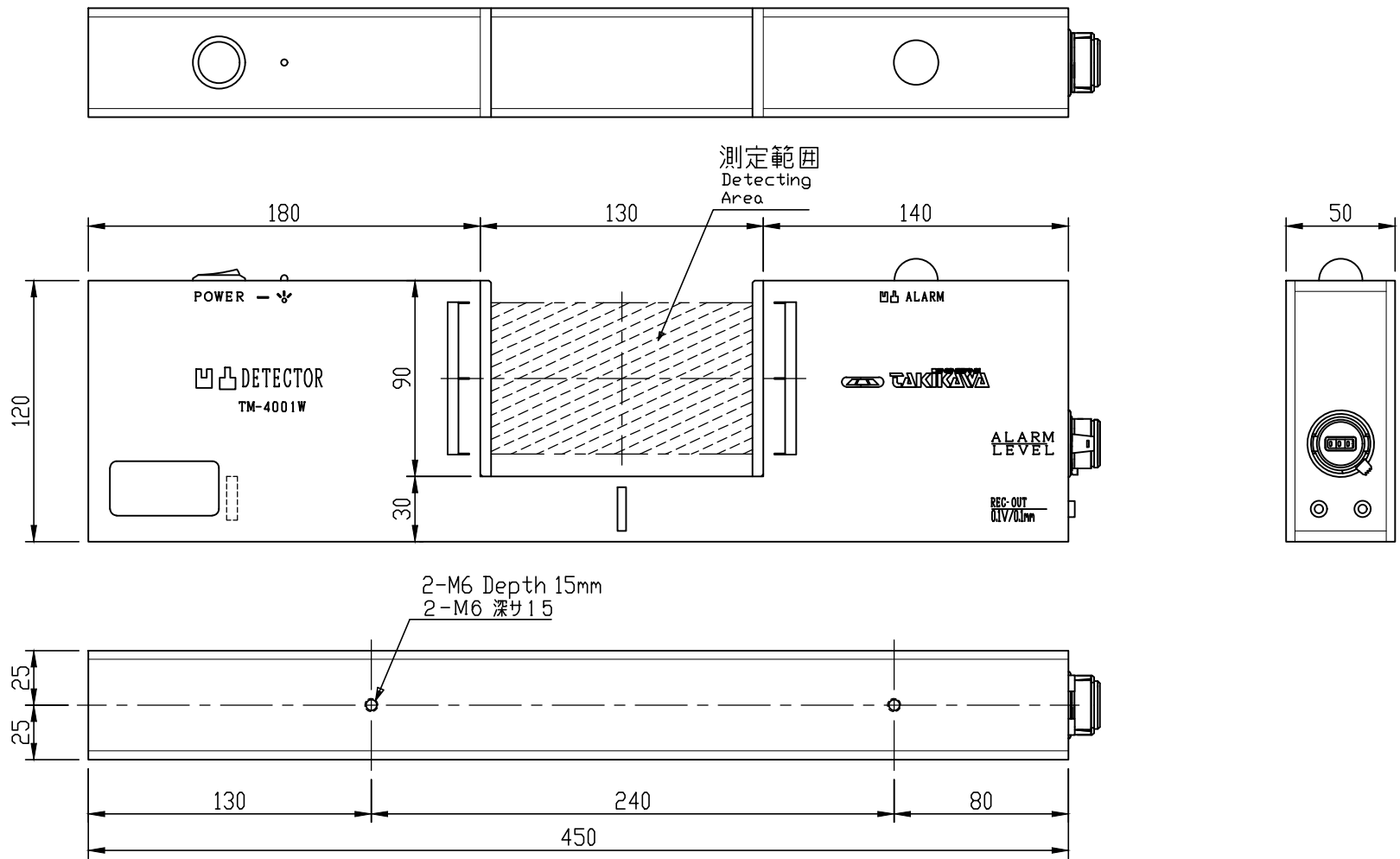
TM-4001 外形図 OutLine Drawing
