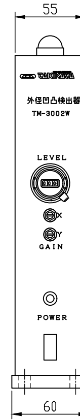
TM-3002W 外形図 Outline Drawing
