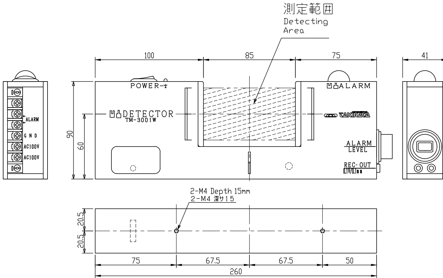
TM-3001W 外形図 Outline Drawing
