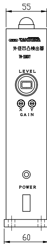
TM-1100XY 外形図 OutLine Drawing
