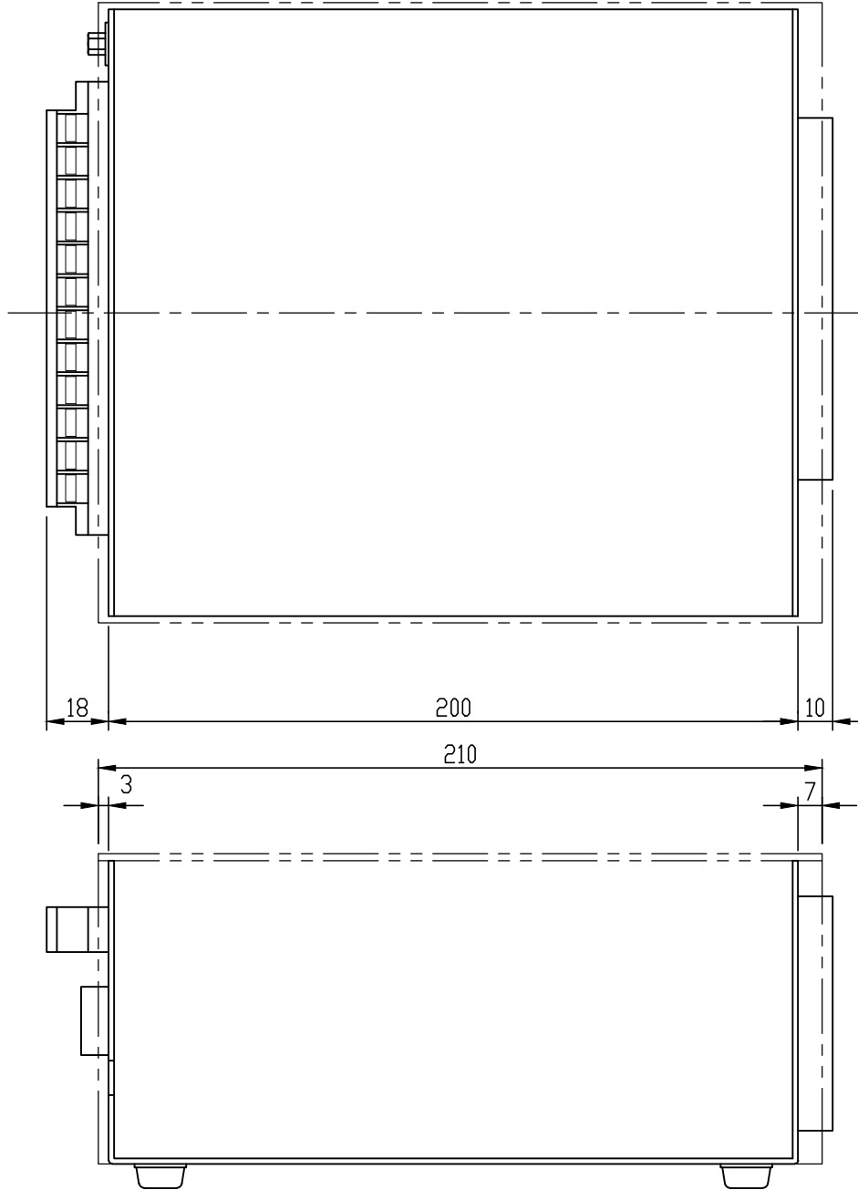
RS-PRINTER 外形図 OutLine Drawing
