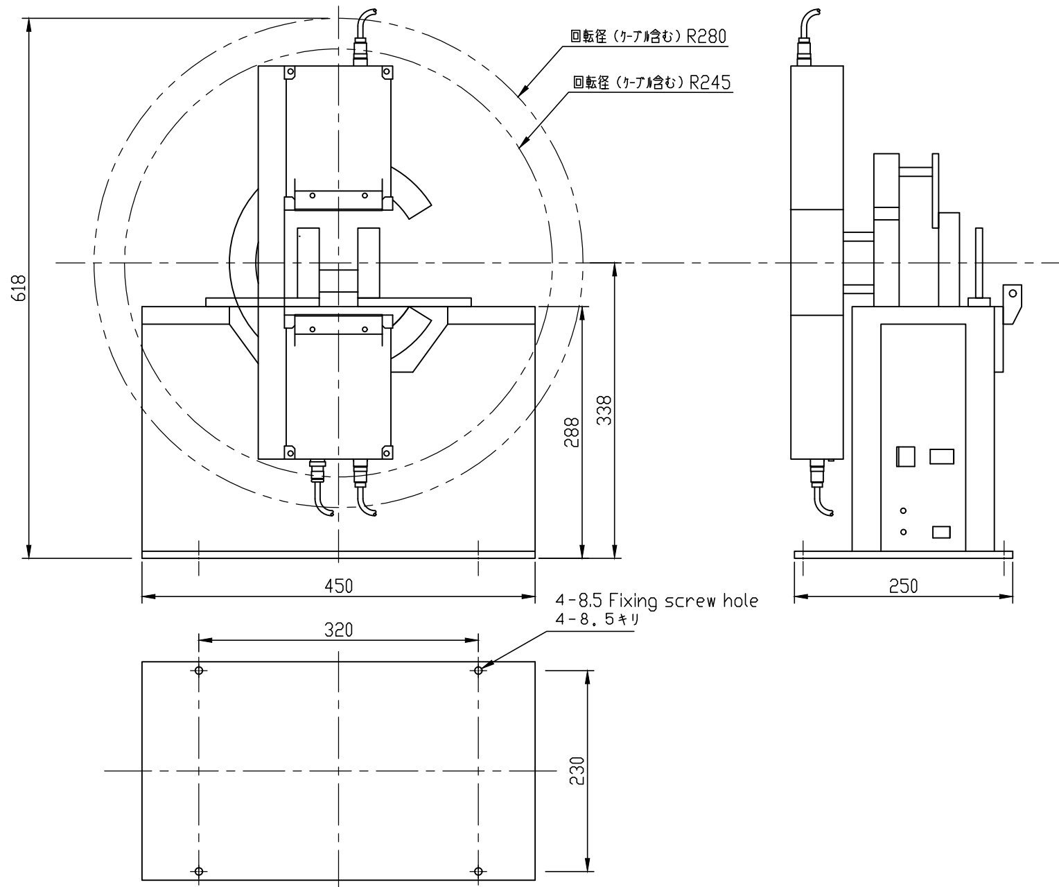
LDM-704A 外形図 OutLine Drawing
