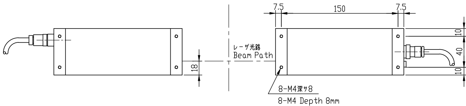
LDM-304H-SP/304HS-SP 外形図
