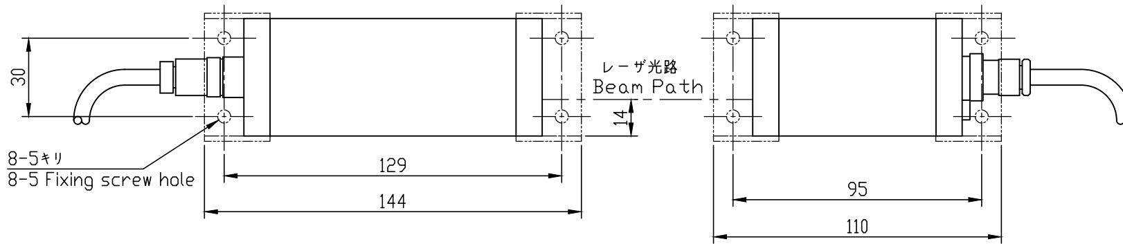
LDM-303H-SP/303HS-SP 外形図 OutLine Drawing
