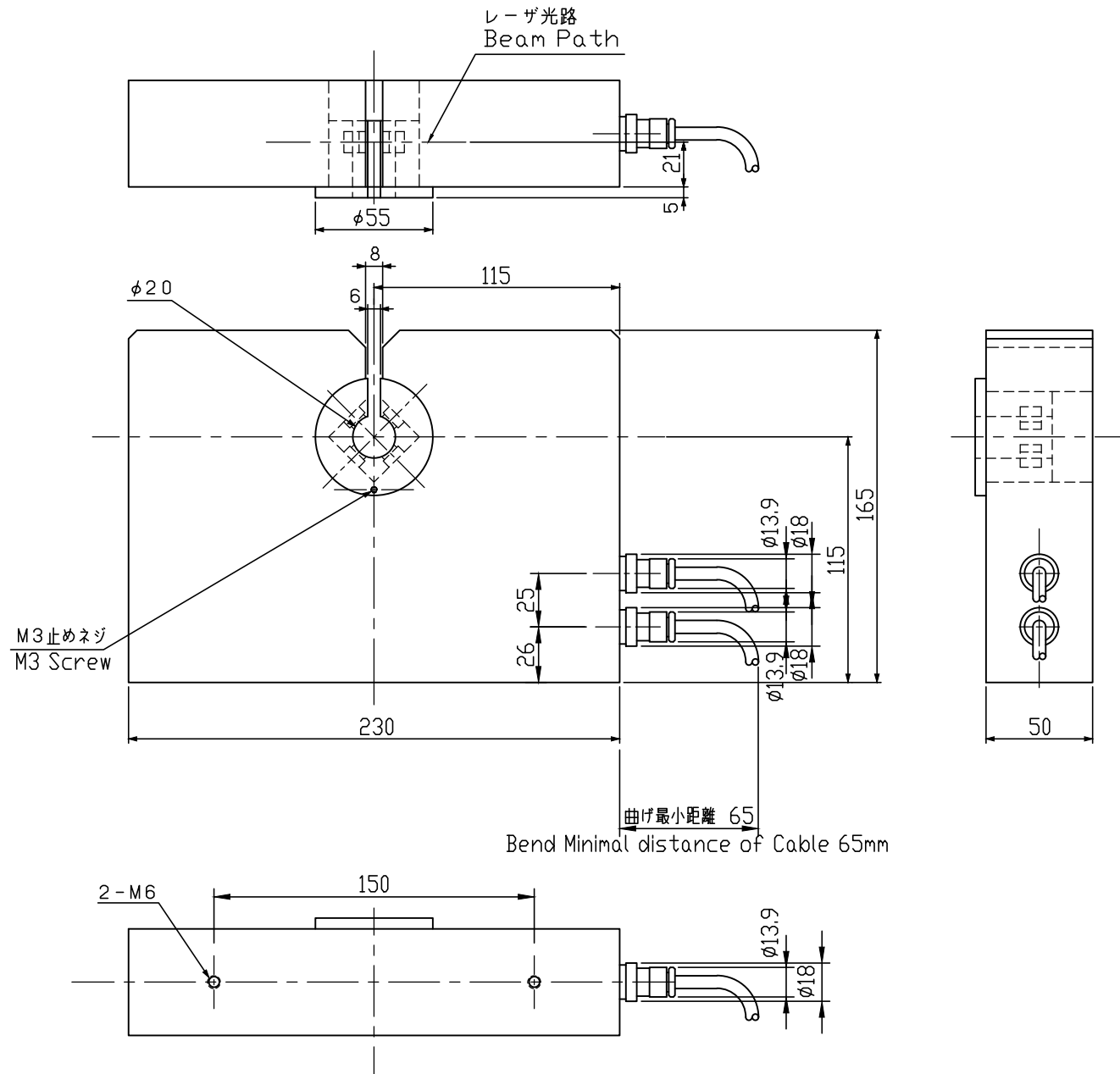
LDM-302H-XY 外形図 Outline Drawing
