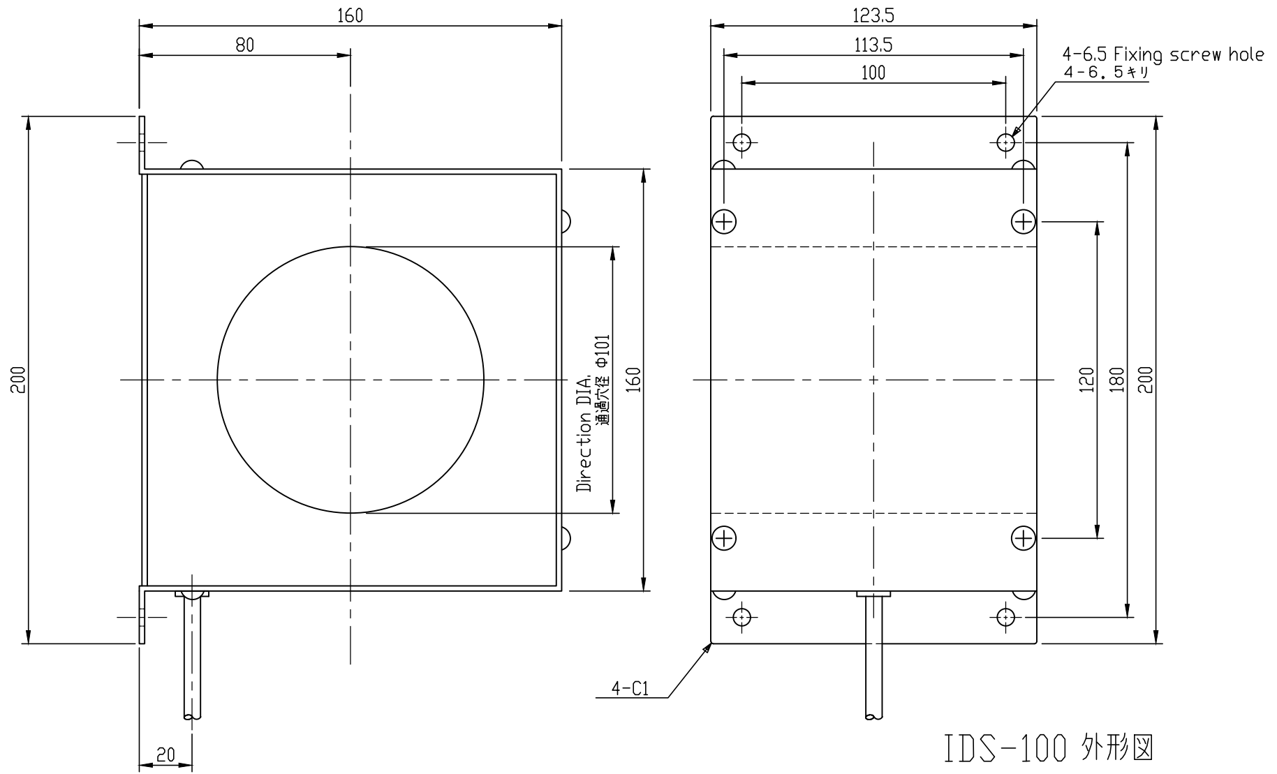
Outline Drawing
