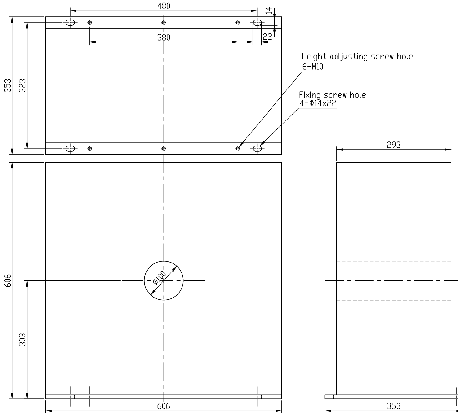
EM-304B 外形图 Outline Drawing
