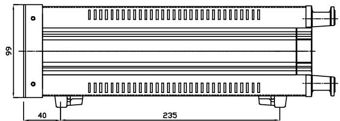
DC-1000K 外形図 OutLine Drawing
