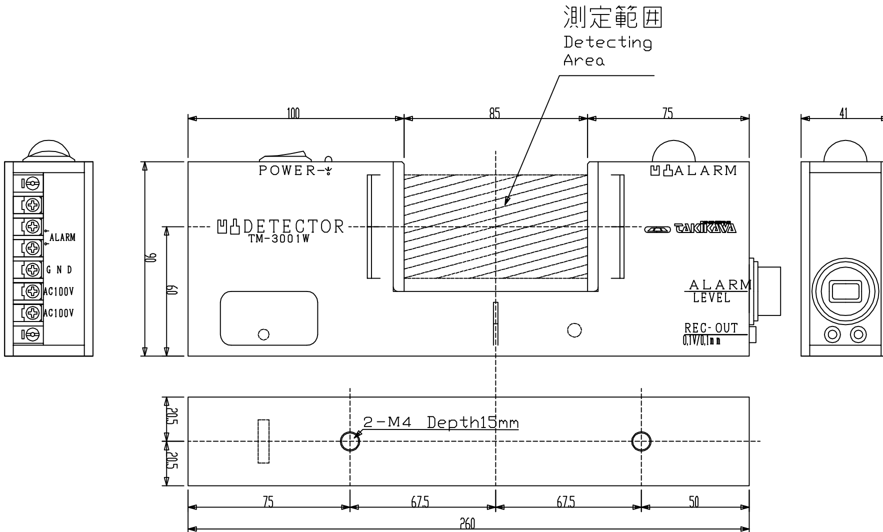
TM-3001W OutLine Drawing 外形図
